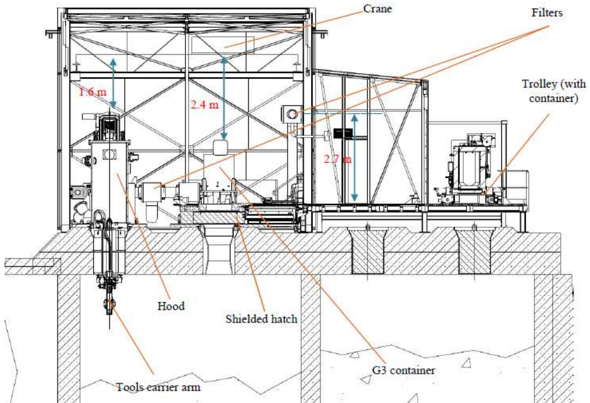
Figure 2.2.1-13. RU3 (middle cross-section shown)
